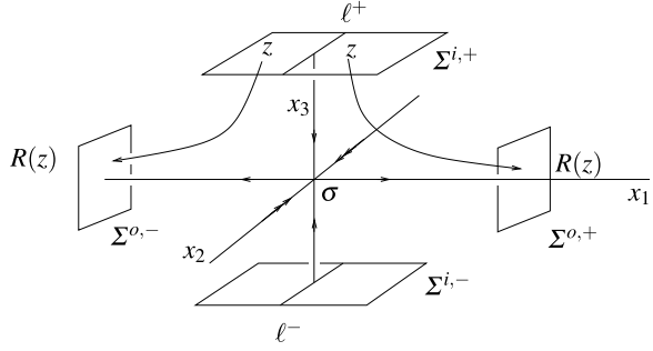
Fig. 5.3 Cross-sections near a Lorenz-like equilibrium
