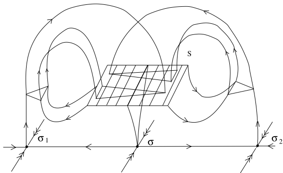
Fig. 9.1 A modified geometric Lorenz attractor
