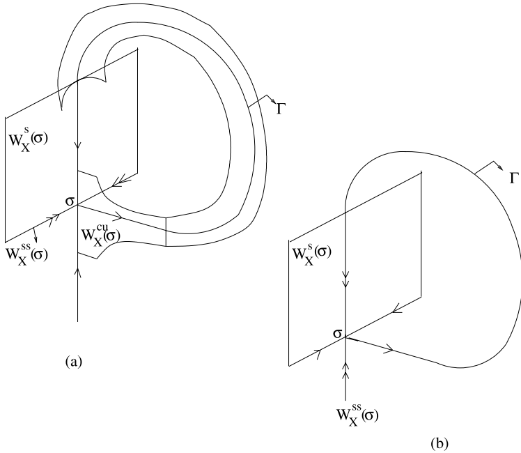
Fig. 3.14 a Inclination-flip. b Orbit-flip
