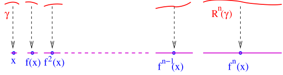
Fig. 7.8 Hyperbolic times and projections
