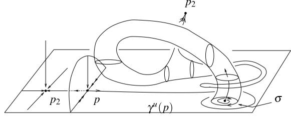
Fig. 3.5 Producing a unique tangency
